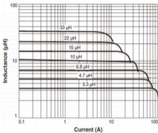
LvsCurrent
