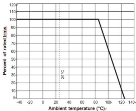
Irms Derating
