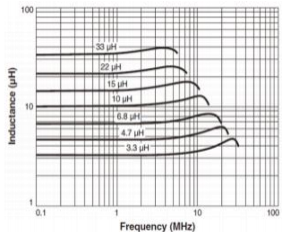
LvsFrequency
