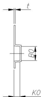
SECTION B-B'
