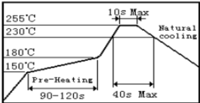
回流焊曲线 Reflow soldering profile
