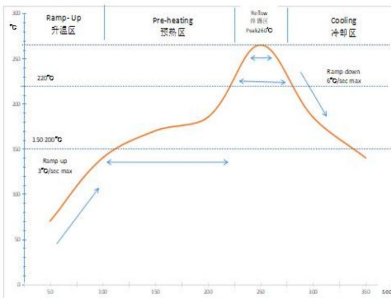
REFLOW PROFILE
