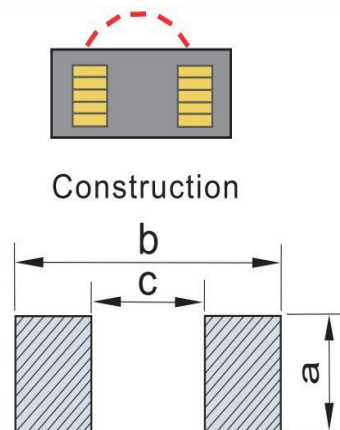
Land patterns
