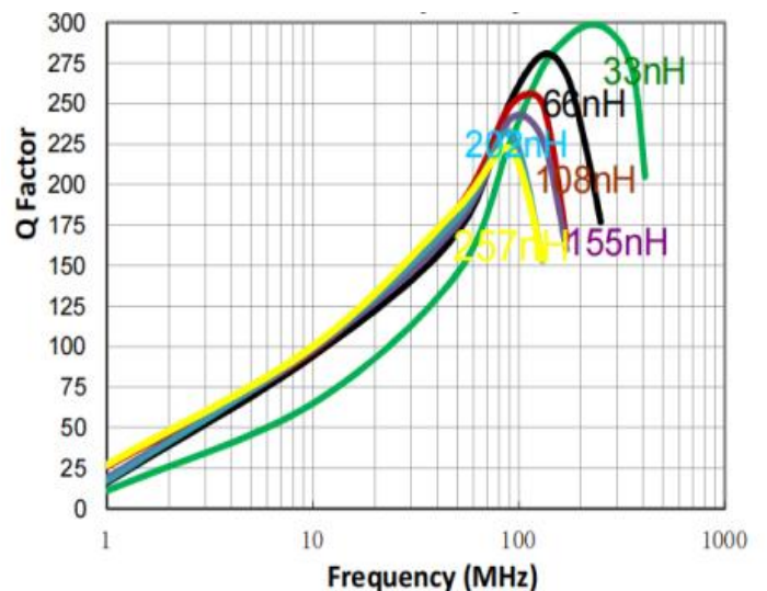
CS2014 Q VS Frequency
