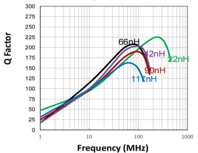
CS1212 Q VS Frequency
