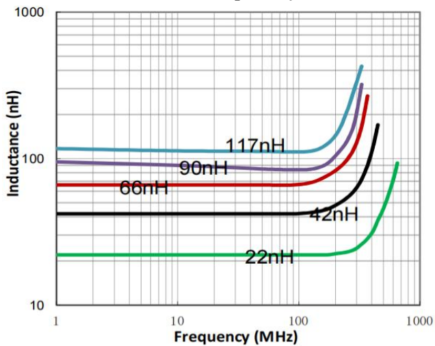
CS1212 L VS Frequency
