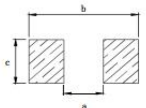
Recommend Land Pattern
